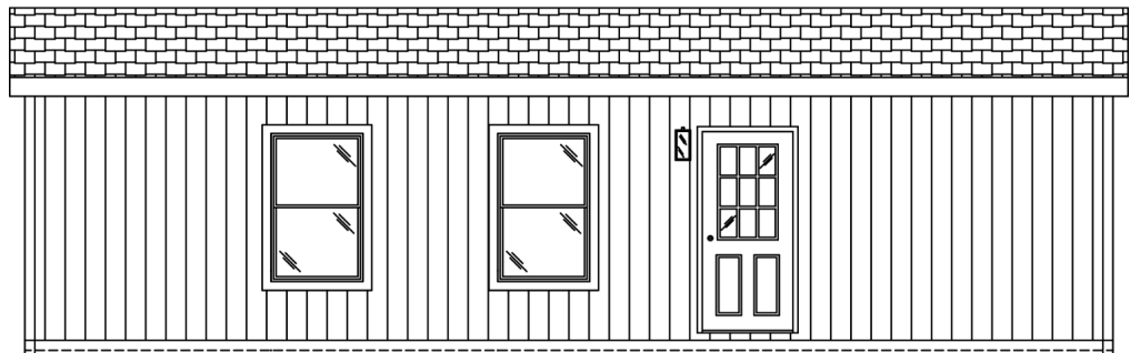
REAR SIDEWALL
